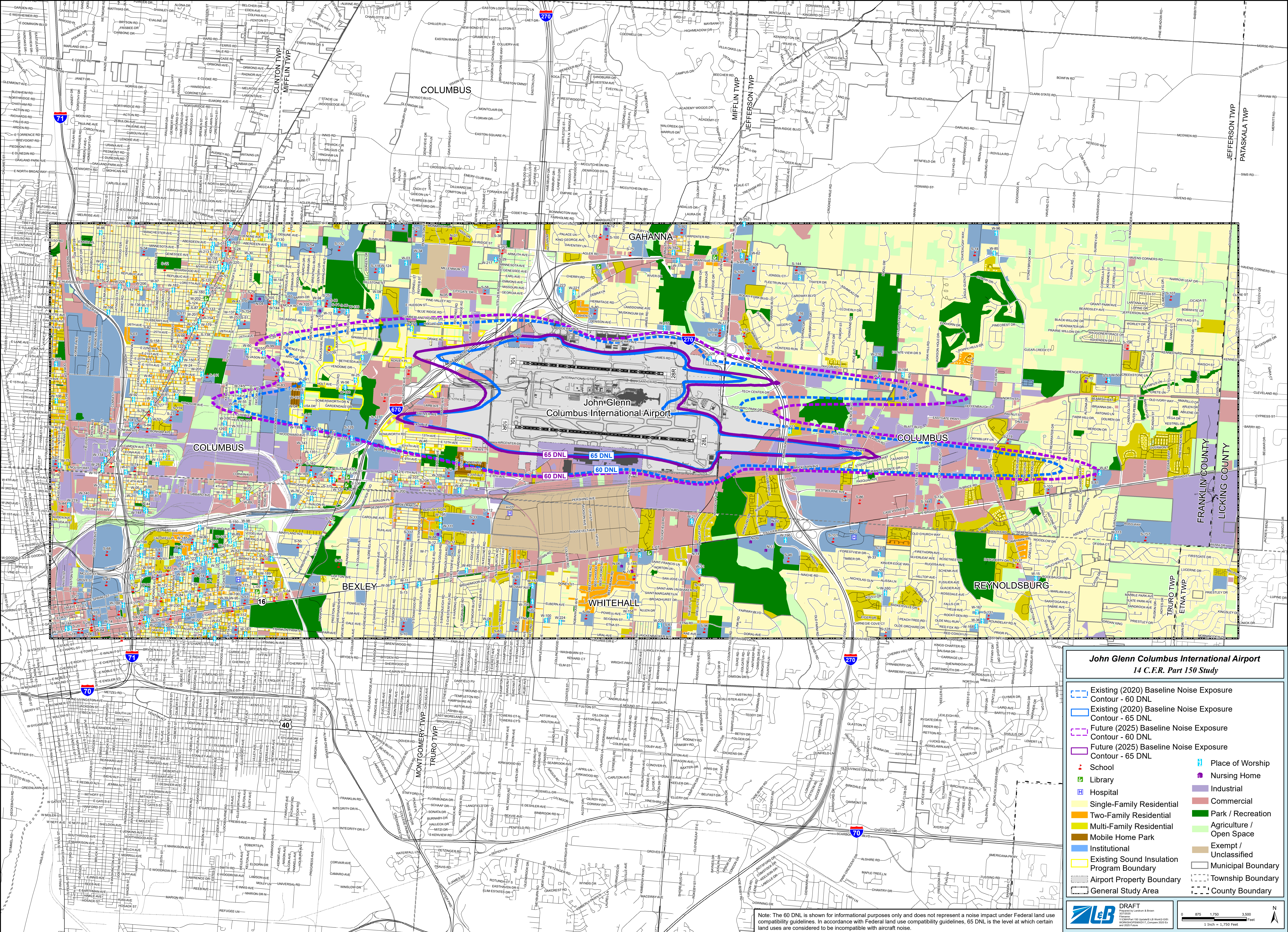
Comparison of Existing (2020) and Future (2025) Baseline Noise Exposure Contours
